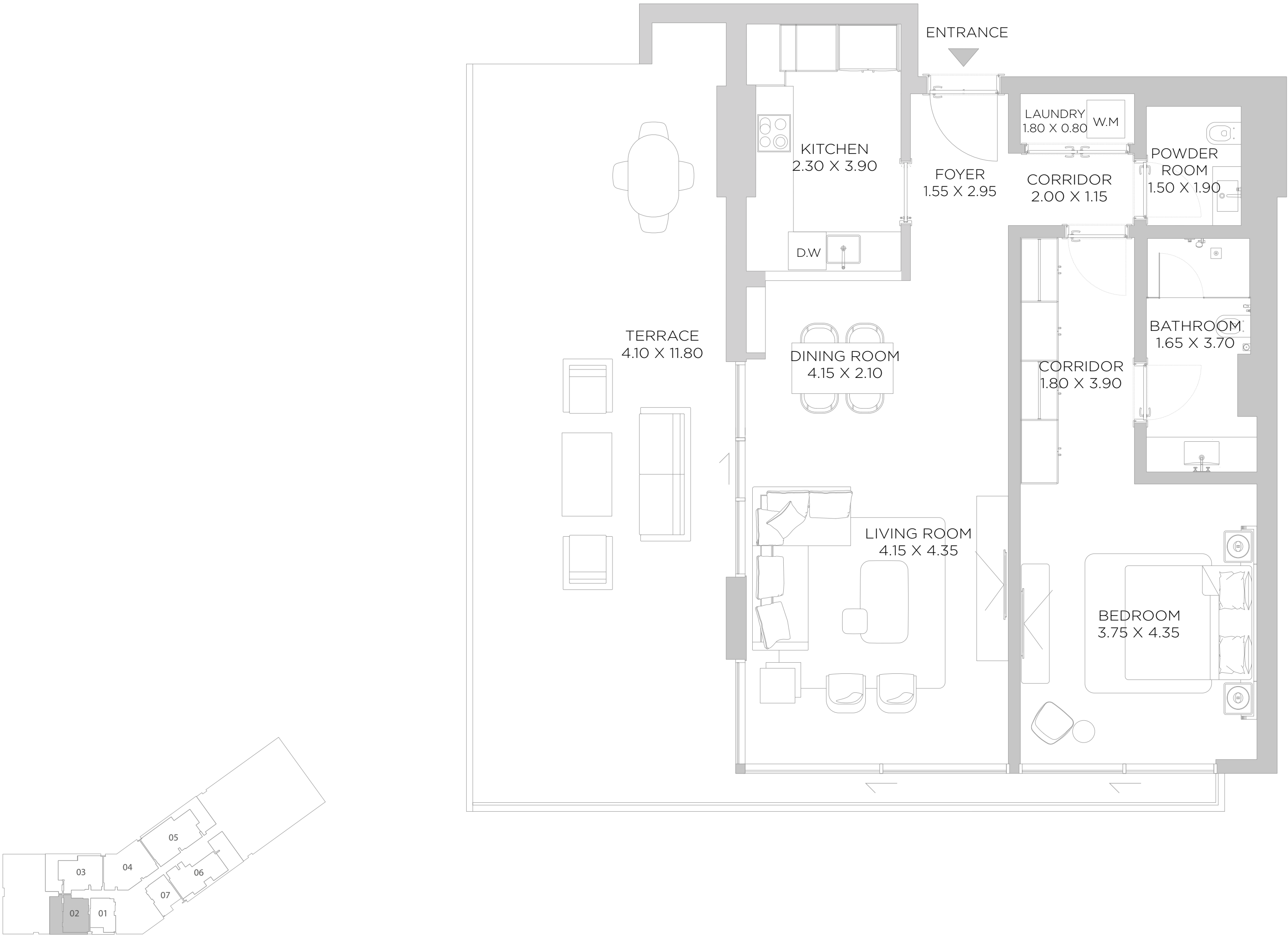
EIGHTH FLOOR PLAN
