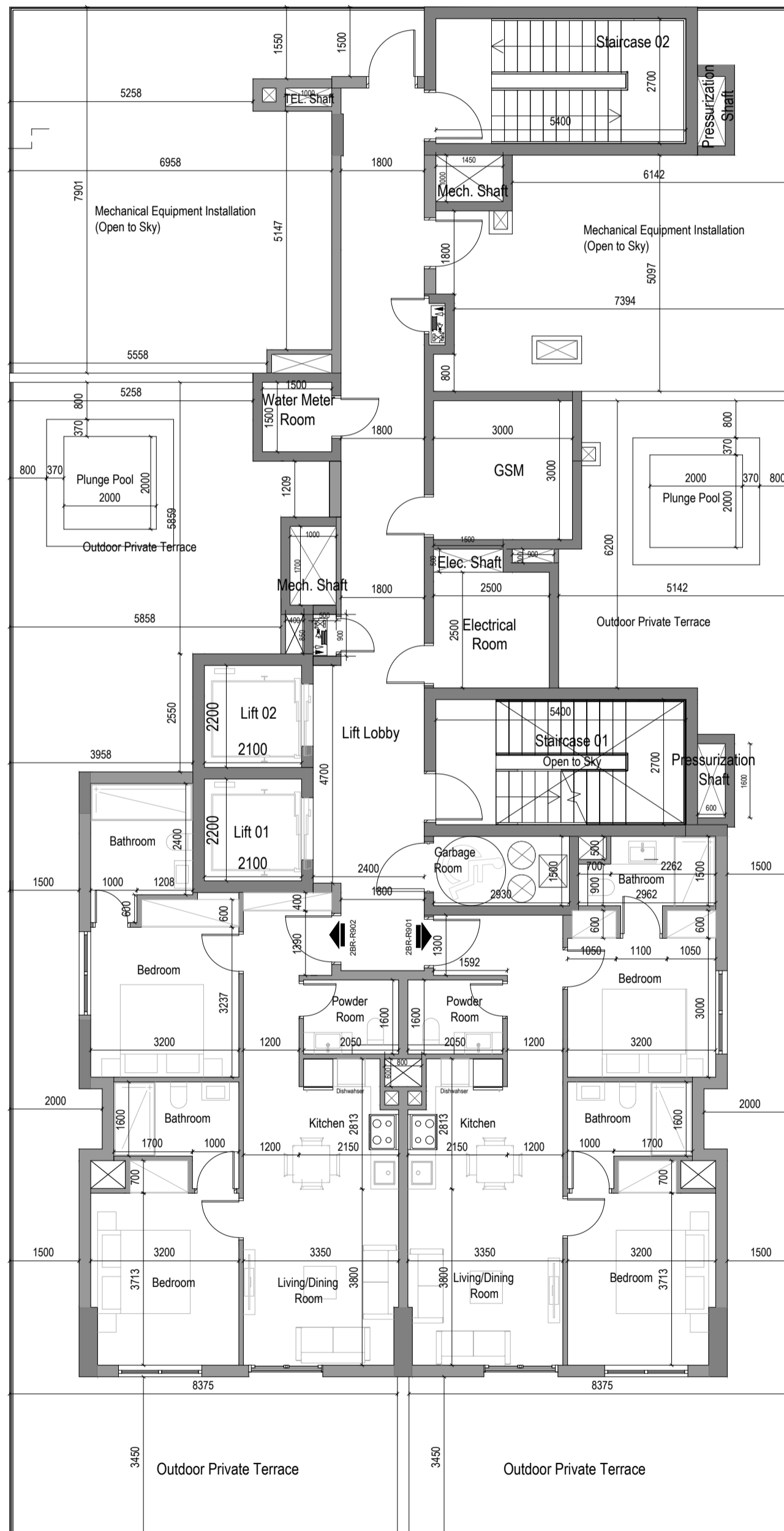
Roof Floor Plan
