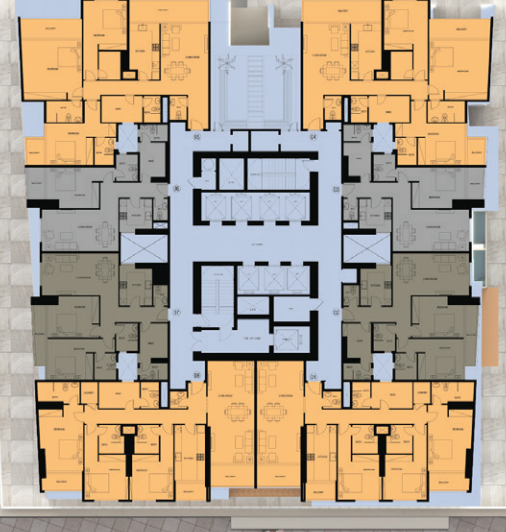
11th, 21st, 31st, 41st FLOOR PLAN SCALE: 1:100
