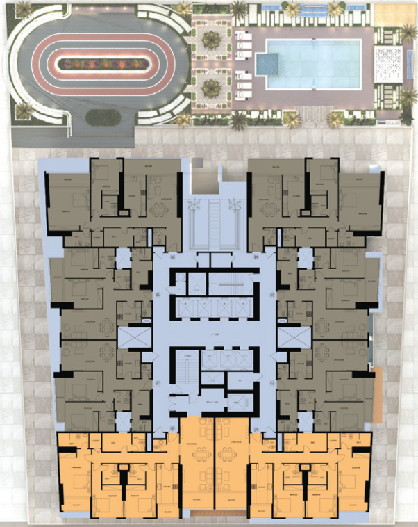
12th to 14th, 22nd to 25th, 32nd to 34th, 42nd to 45th FLOOR PLAN SCALE: 1:100
