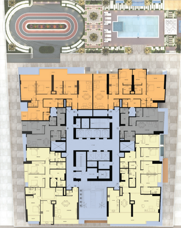
47th FLOOR PLAN SCALE: 1:100
