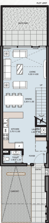
GROUND FLOOR
