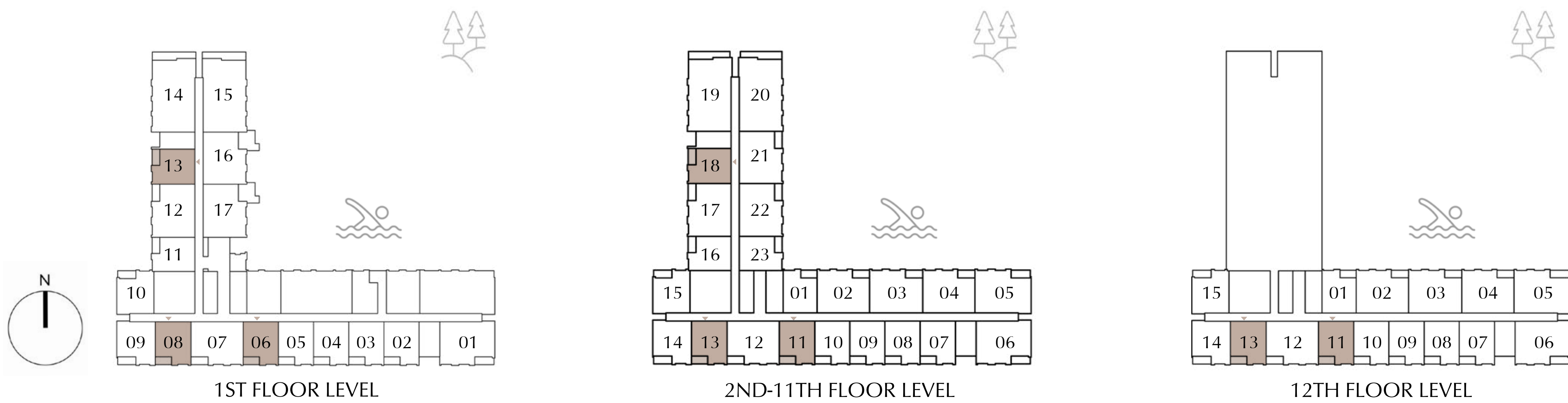
KEY PLAN
