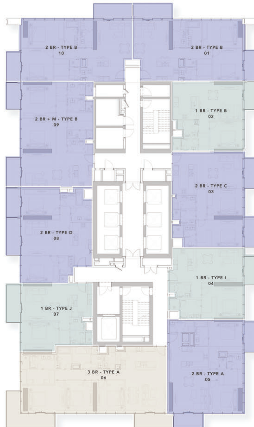
LEVEL 18-19 & 23-30 TYPICAL FLOOR PLAN
