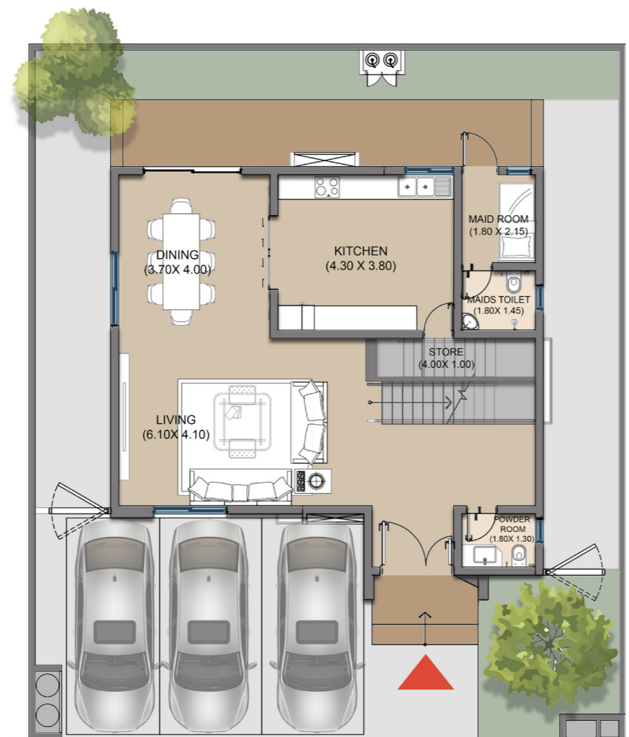
GROUND FLOOR PLAN - 96.70 SQ.M
