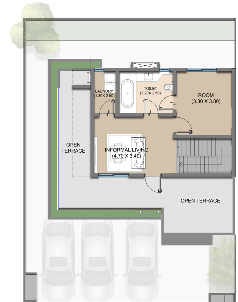
PENTHOUSE FLOOR PLAN - 55.90 SQ.M
