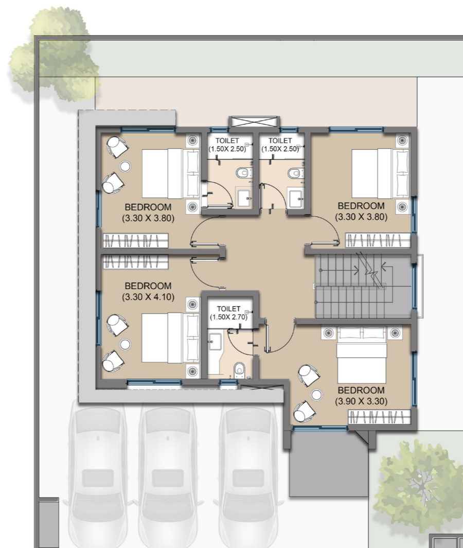
FIRST FLOOR PLAN - 96.70 SQ.M
