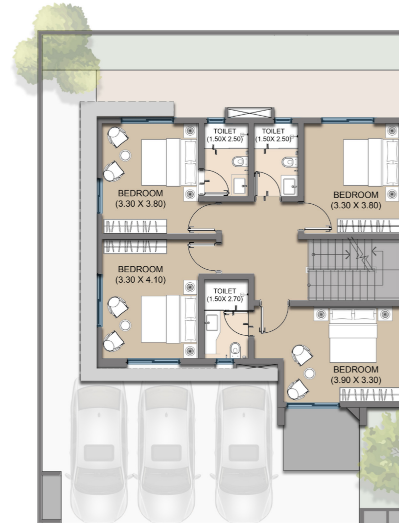
FIRST FLOOR PLAN - 96.70 SQ.M
