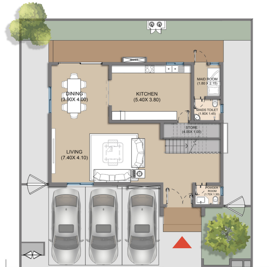
GROUND FLOOR PLAN - 107.60 SQ.M
