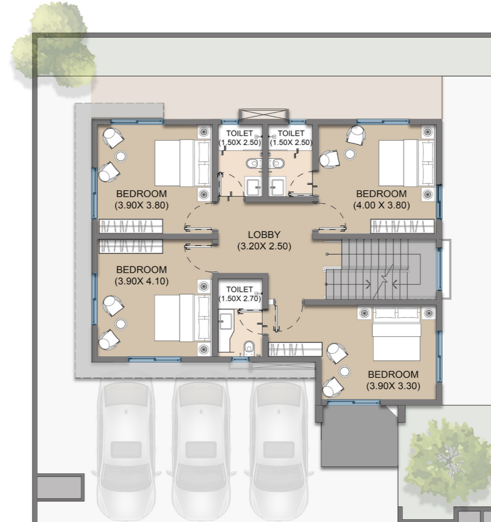
FIRST FLOOR PLAN - 107.60 SQ.M
