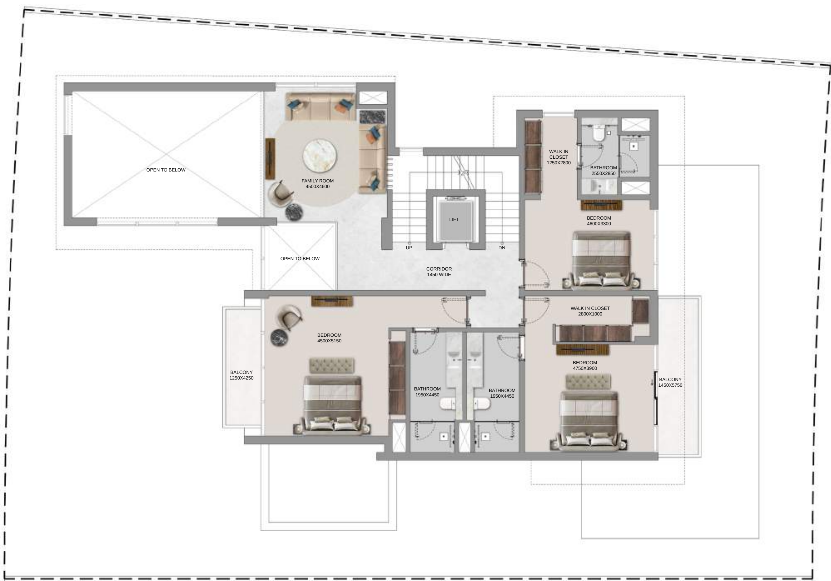
FIRST FLOOR
