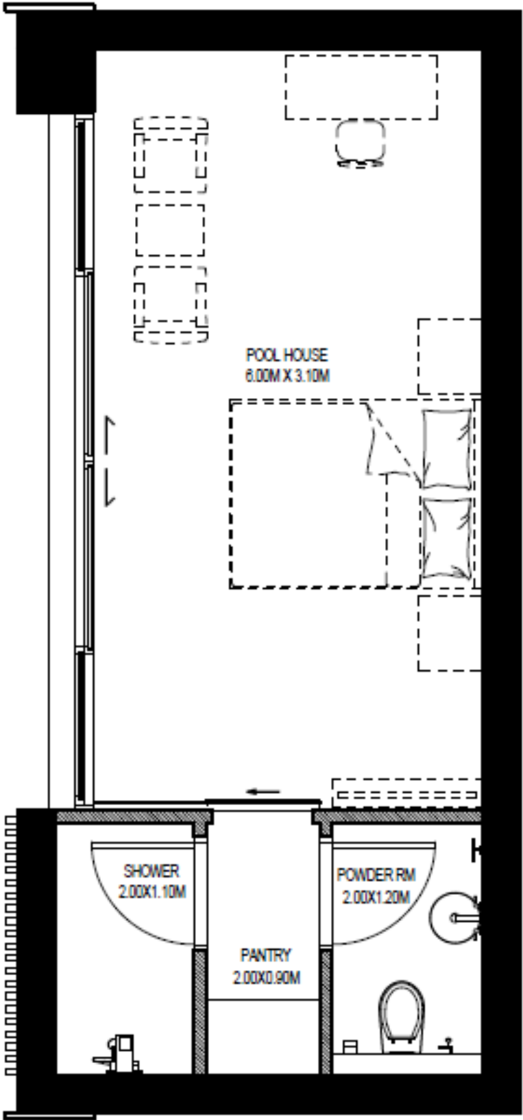
POOL HOUSE
