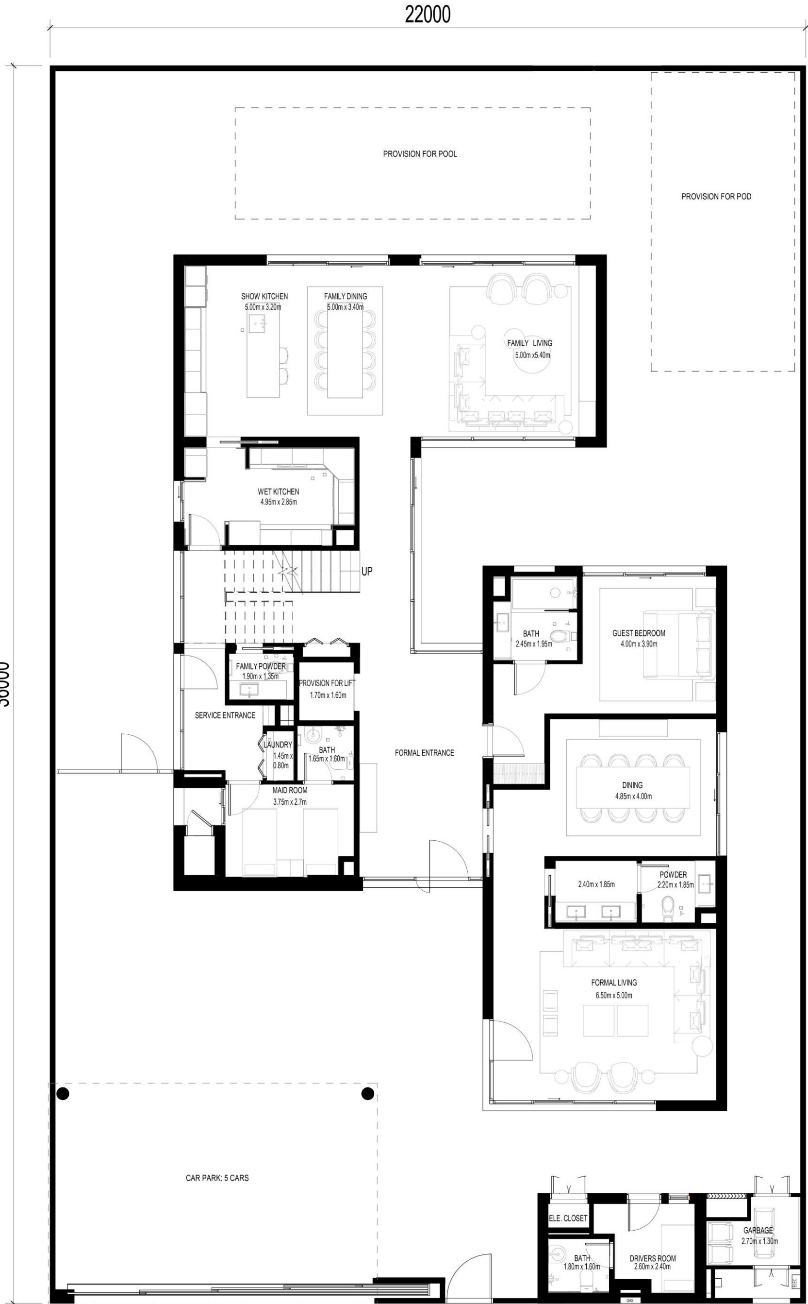
GROUND FLOOR
