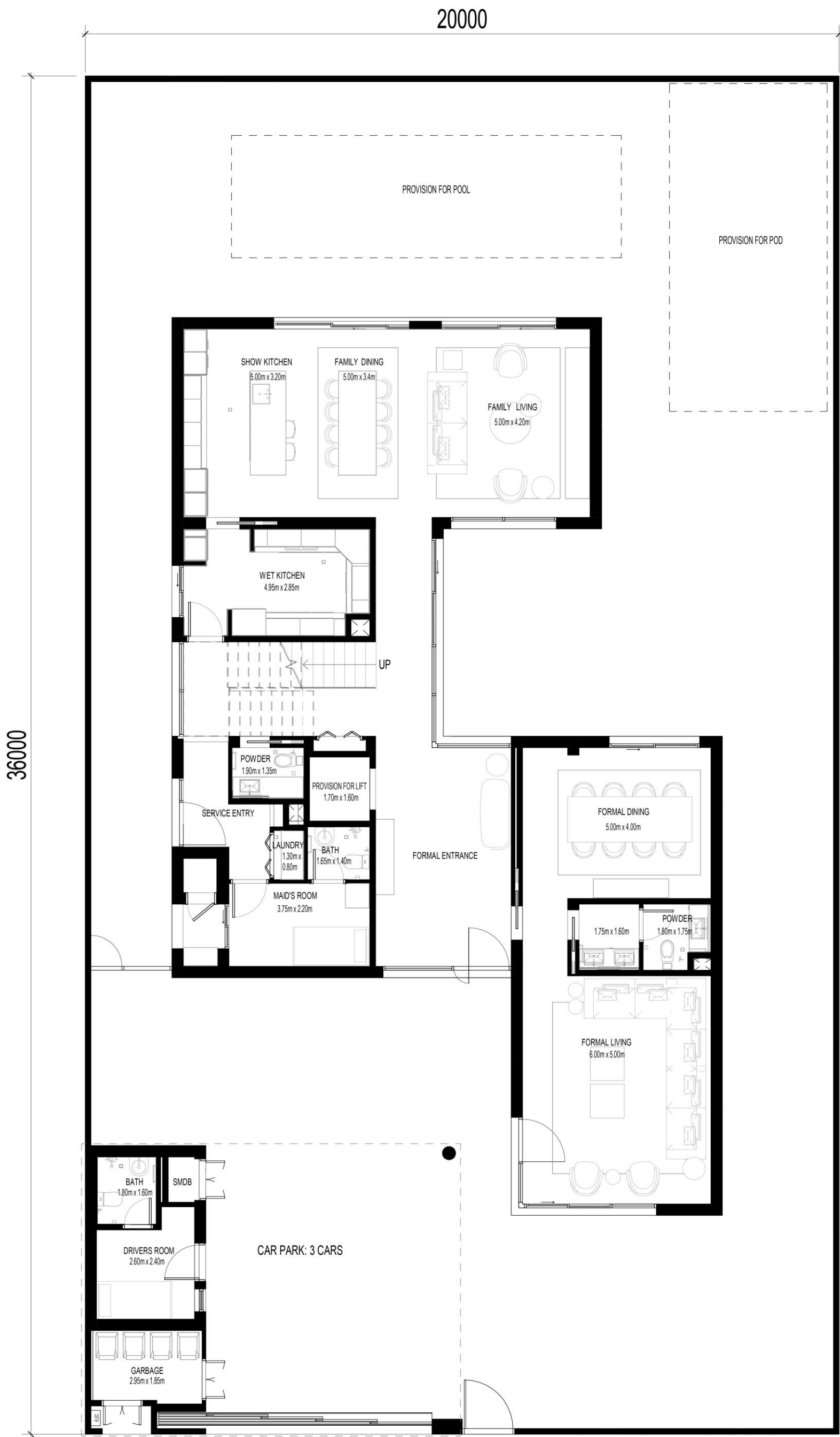
GROUND FLOOR
